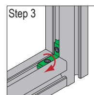
tighten L2 top thread 锁紧L2顶丝
