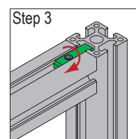
tighten L2 top thread 锁紧L2顶丝
