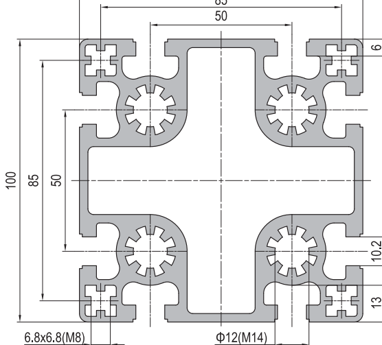
100x100 8 slots 100x100 8槽
