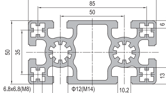
50x100 6 slots 50x100 6槽
