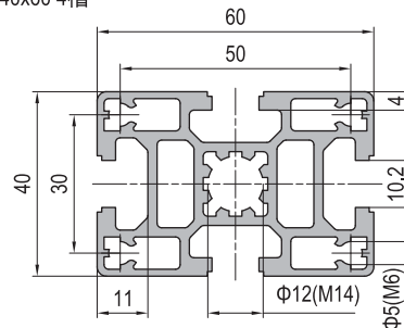
40x60 4 slots 40x60 4槽
