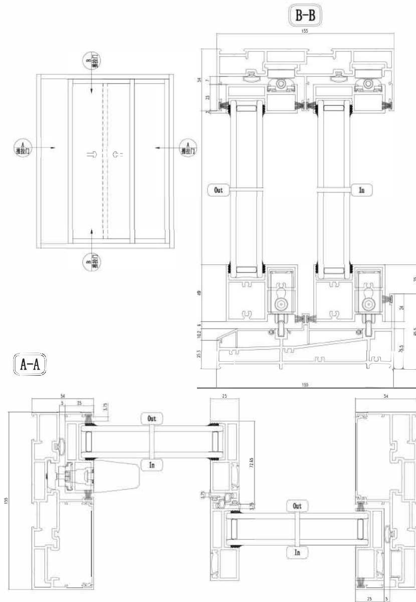
➡ JP-GKT155AM Sliding door- Non Thermal Break
