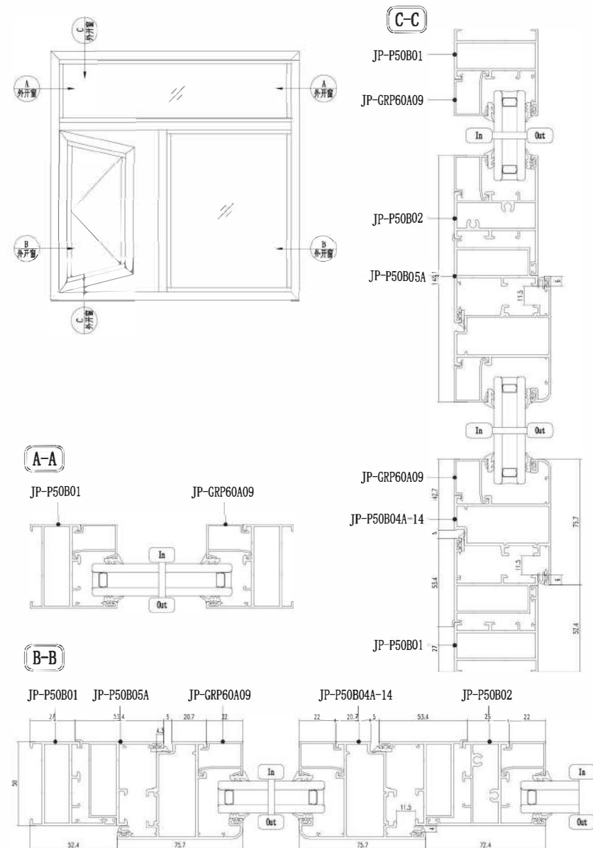
JP-P50B Casement Window & Door - Non Thermal Break
