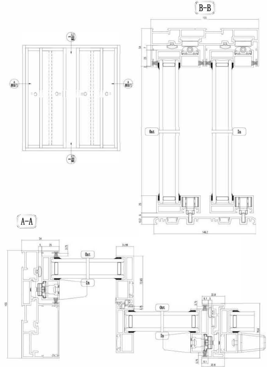
JP-GKT155AM Sliding door- Non Thermal Break ◀
